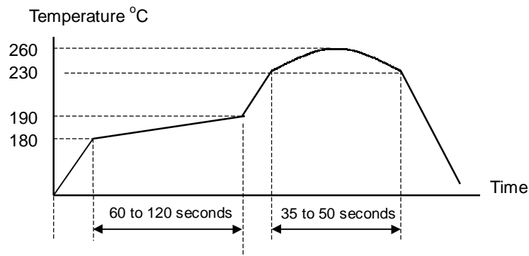
[Recommended temperature profile of a far-infrared heater, hot air reflow]
